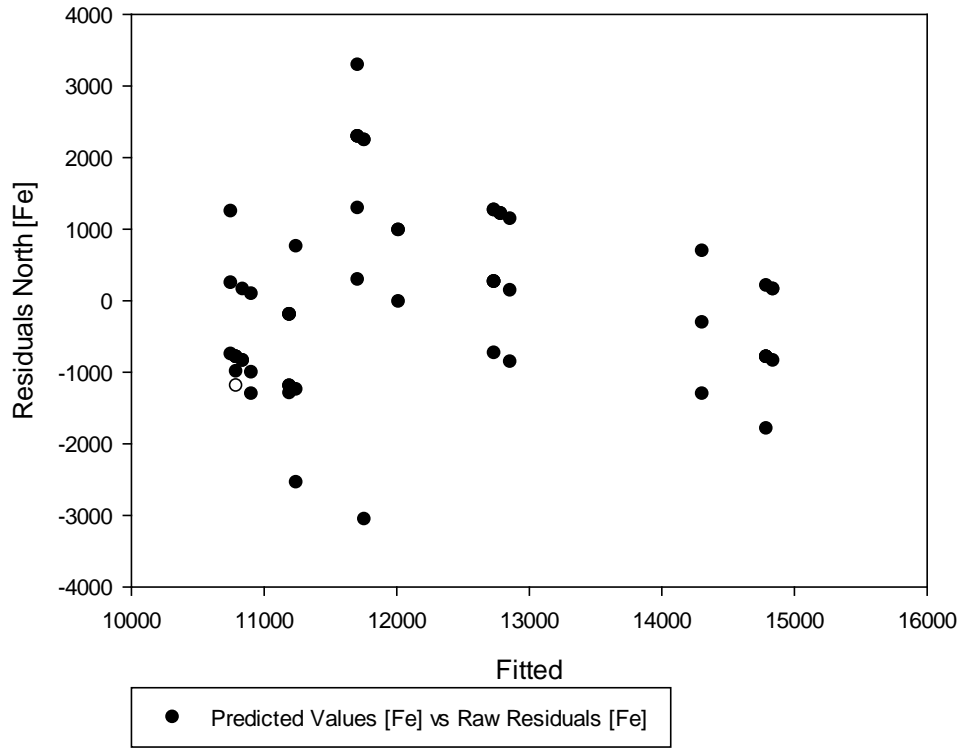
Residuals vs Fitted: North Transect Iron Conc.
