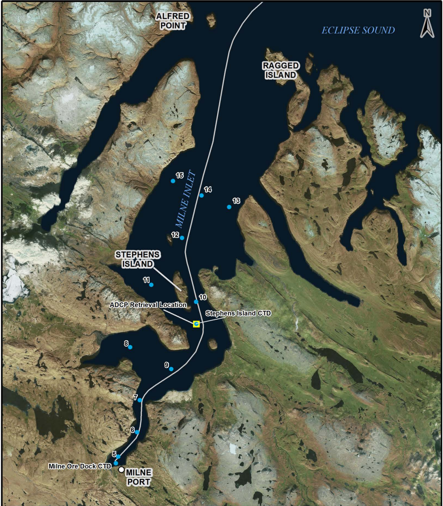
FIGURE ID:070-025-1-012 Locations of CTD Profiles and ADCP Retrieval in Milne Inlet, 2016
