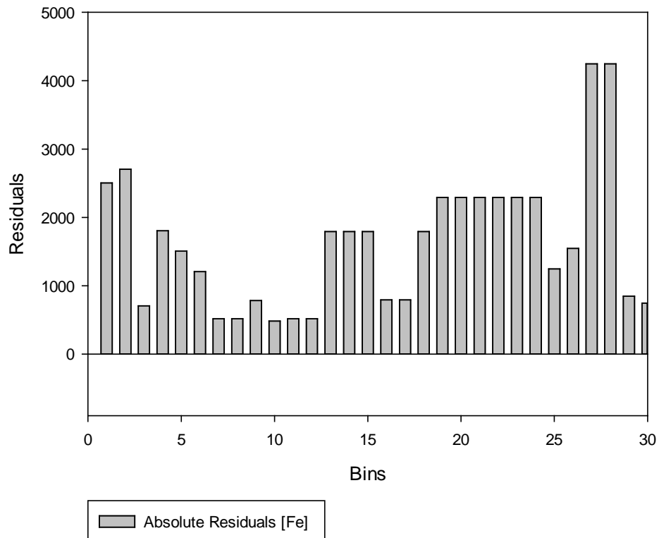
Histogram of residuals: West Iron Conc.
