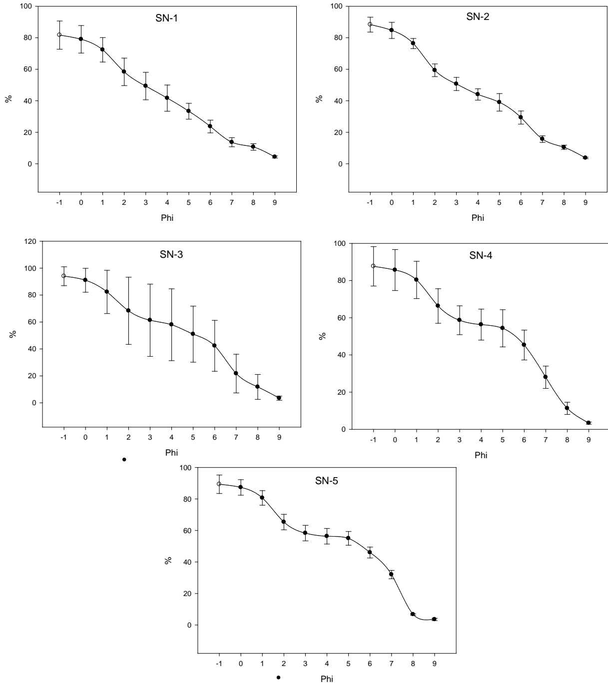
Figure 3.9 Phi Scale Particle Size Distribution for the North Transect (with standard deviation).
